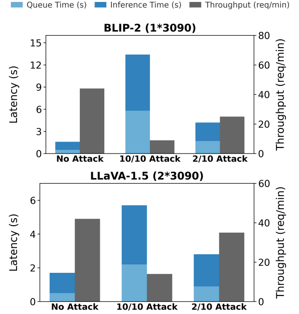
Fig. 1: Attack on Real-world LVLMS Serving System (SGLang). 10/10 attack and 2/10 attack mean 10 of 10 clients and 2 of 10 clients attack the serving system. Client latency, generally marked in blue, consists of queue and inference time.
